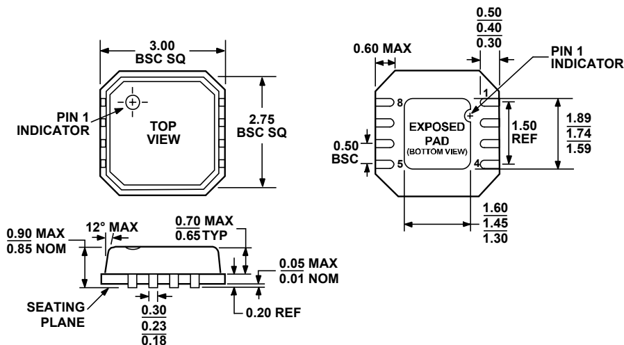
Figure 59. 8-Lead Lead Frame Chip Scale Package [LFCSP_VD] 3 mm x 3 mm Body, Very Thin, Dual Lead (CP-8-2)
